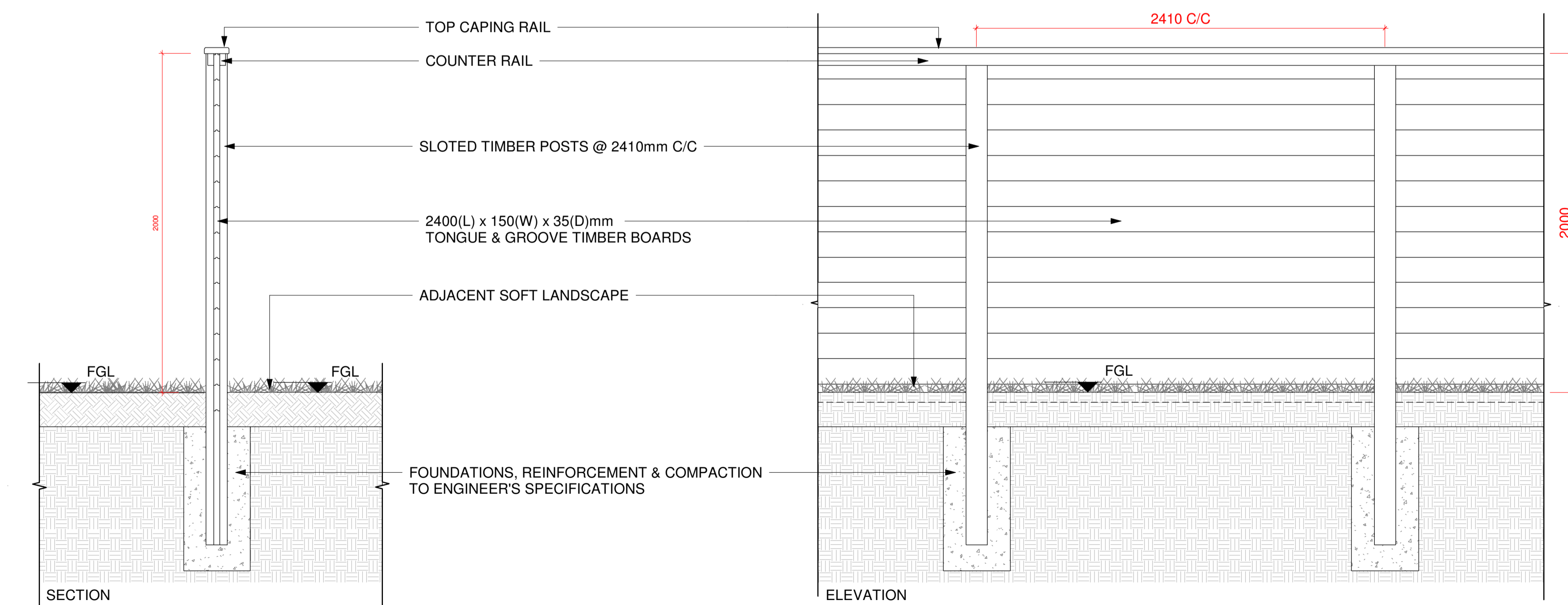
SECTION 2 2m HIGH ACOUSTIC FENCING SCALE: 1:20 @A1
