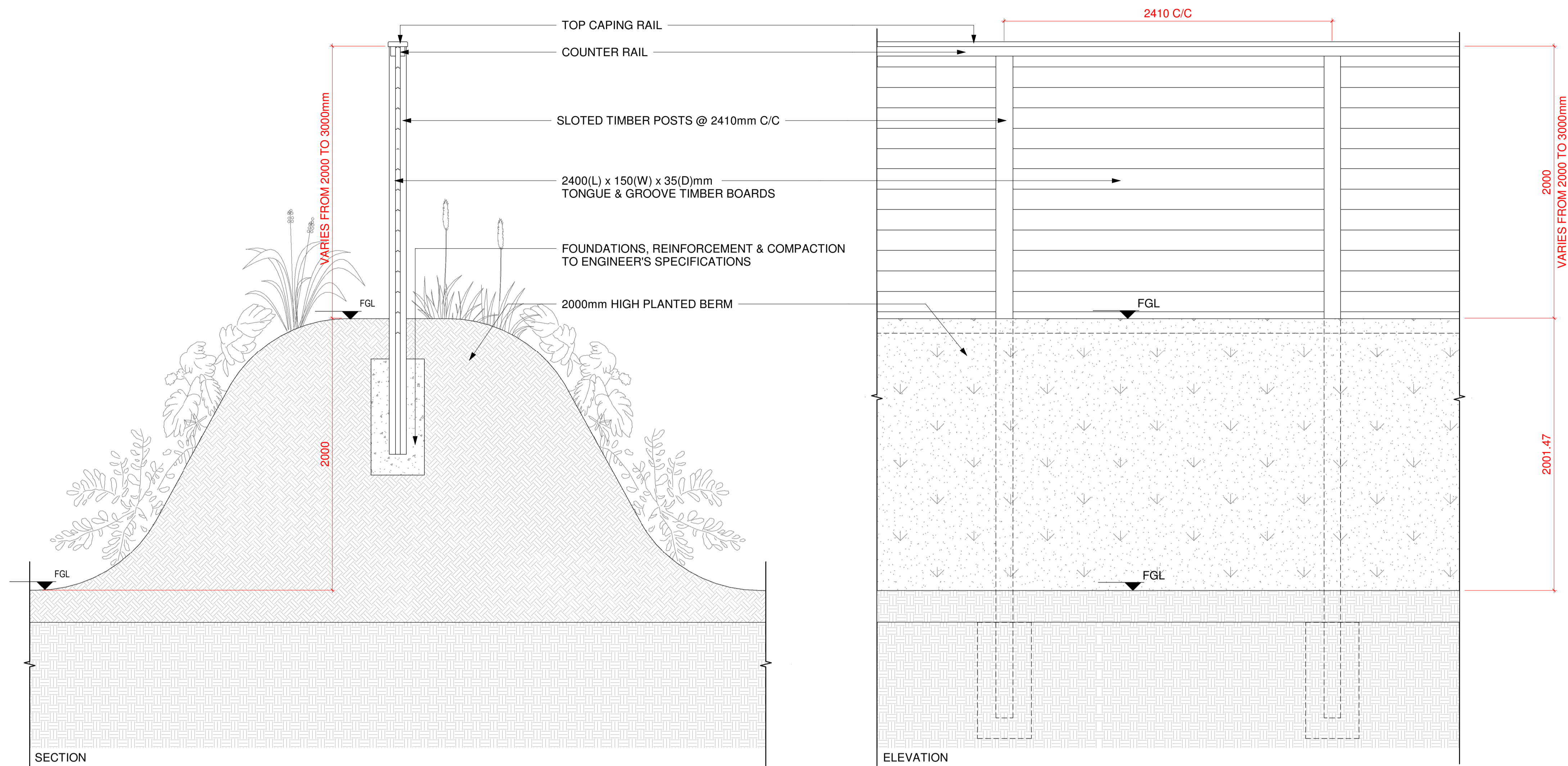
SECTION 1 TYPICAL DETAIL: 2m HIGH ACOUSTIC FENCING ON 2m HIGH PLANTED BERM SCALE: 1:20 @A1
